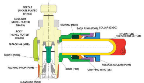
Figure 1.4 Diagram of Flow Controller
