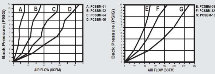
FLOW CHARACTERISTICS - PNEUMATIC EXHAUST MUFFLER
